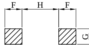
( PCB Pattern )
